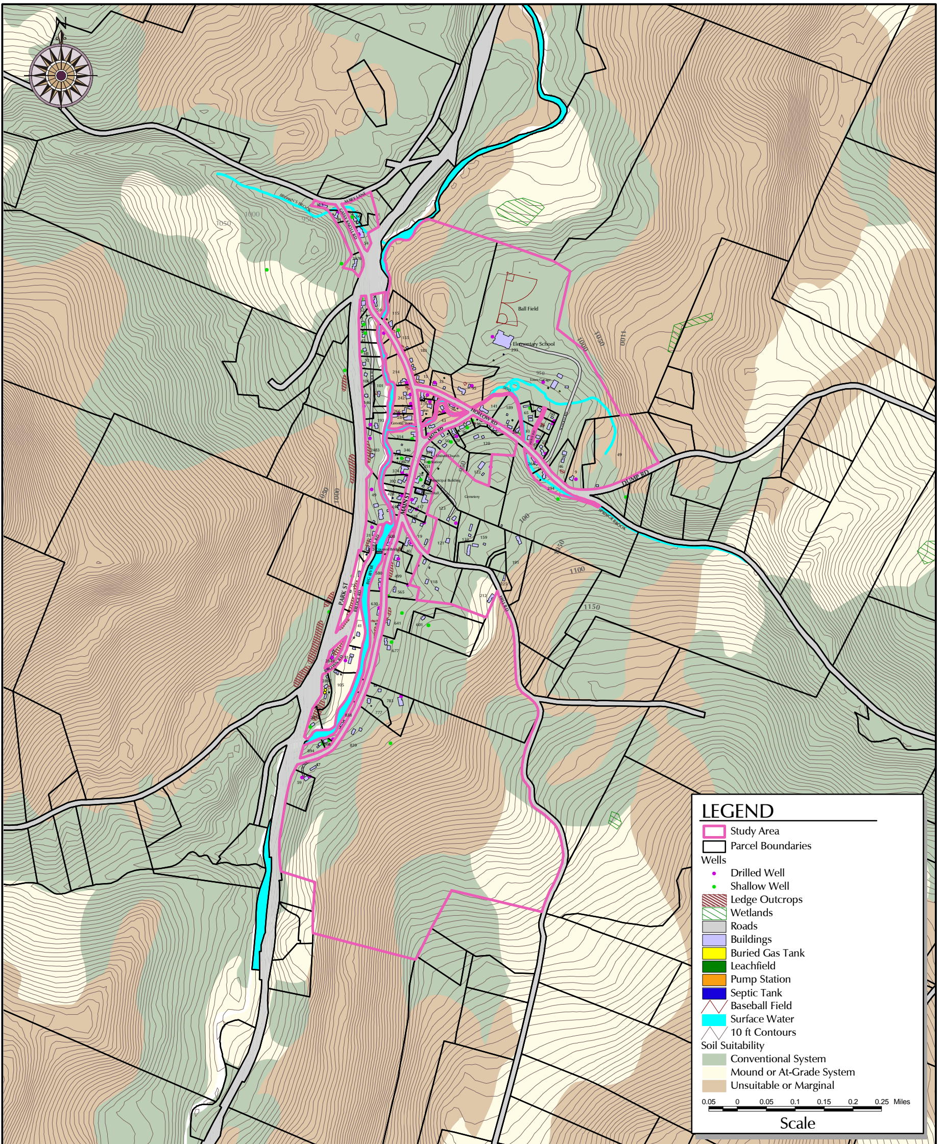
FIGURE 2: ENVIRONMENTAL SENSITIVITIES
